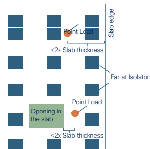
Figure 3: Point loads close to slab edges or openings.
