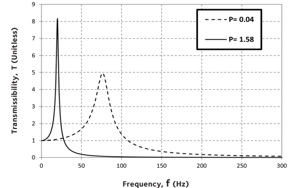
Fig 5.0 Transmissibility at Min and Max working Pressure (P)
