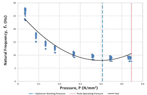
Fig 2.0 Natural Frequency vs. Pressure
