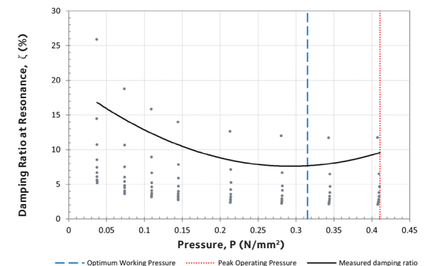
Fig 3.0 Damping Ratio at Resonance vs. Pressure
