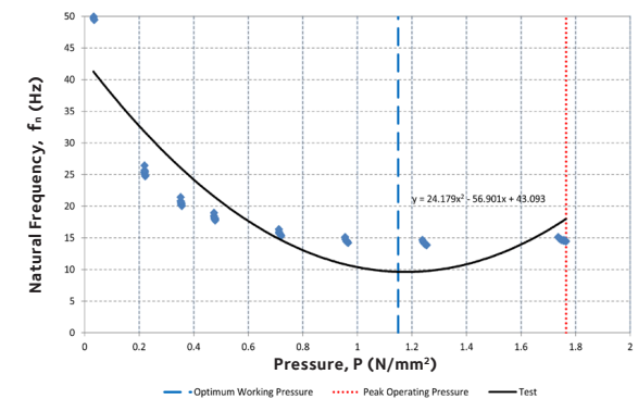
Fig 2.0 Natural Frequency vs. Pressure
