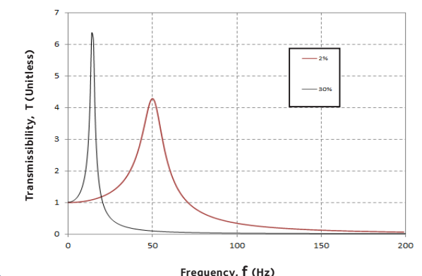
Fig 5.0 Transmissibility at Min and Max working Pressure (P)
