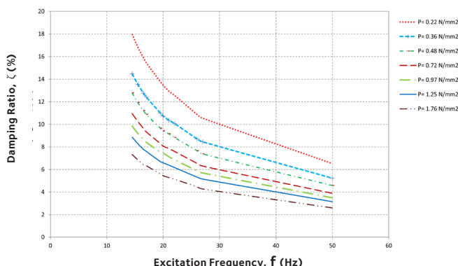
Fig 4.0 Damping Ratio at different Pressure (P) and different Peak-to-Peak Dynamic Amplitudes (X)
