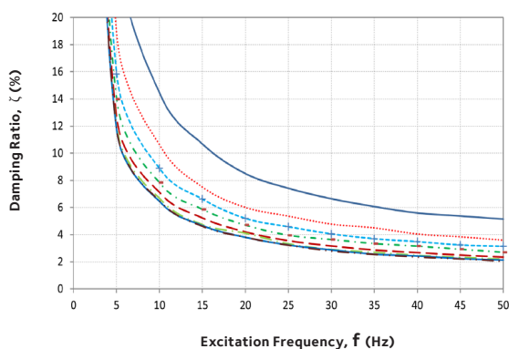
Fig 4.0 Damping Ratio at different Pressure (P) and different Peak-to-Peak Dynamic Amplitudes (X)
