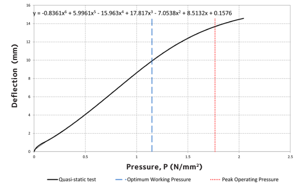
Fig 1.0 Quasi-Static Deflection vs. Pressure
