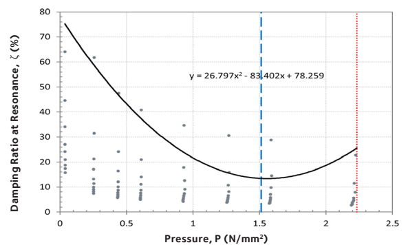
Fig 3.0 Damping Ratio at Resonance vs. Pressure
