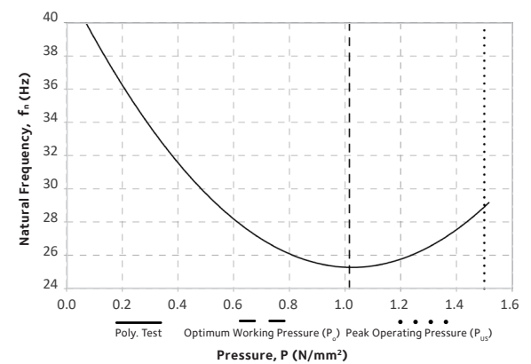
Fig 2.0 Natural Frequency vs. Pressure
