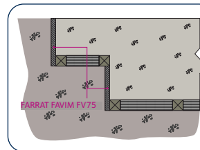
Farrat Favim FV75 used as foundation sidewall isolation
