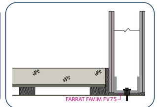
Farrat Favim FV75 used to isolate a lightweight partition
