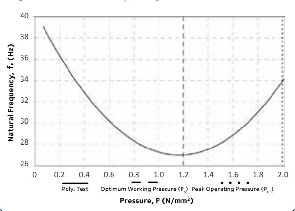
Fig 2.0 Natural Frequency vs. Pressure
